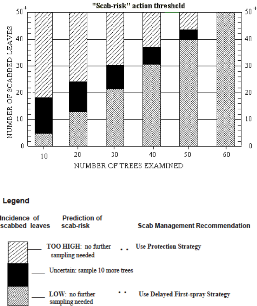
Figure 6.2.1. Sequential sampling chart for determining level of scab risk in an orchard block. Use this chart if sanitation practices will NOT be considered.
